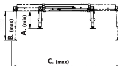
Cylinder Ø 100 mm
